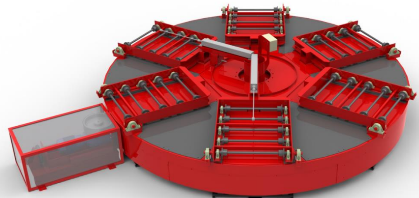
6 Station Carousel for Moulding
