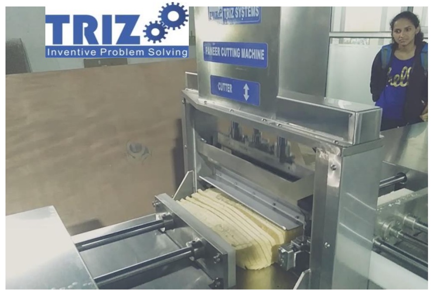
Paneer / Cheese Slice Cutting Machine
