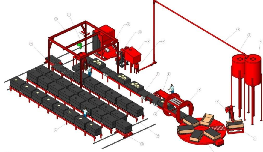
Proposed Plant Layout
